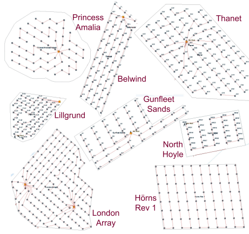
Figure 1: Actual OWFs with uniform distribution of turbines. Obtained from www.4coffshore.com/offshorewind/ .
