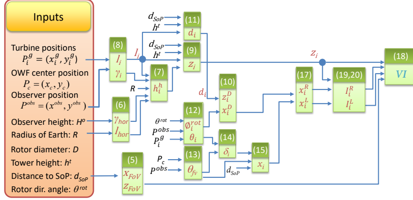
Figure 6: Stream of calculations to obtain the visual impact. Input variables are written in black and intermediate variables, in brown. The expressions linking the variables appear in white
