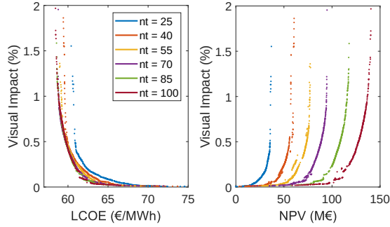
Figure 14: Non-dominated solutions for six different OWF sizes.
