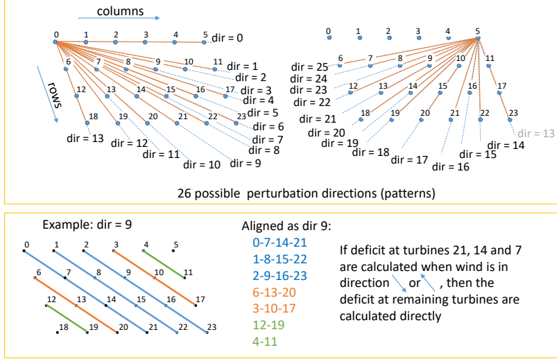
Figure 3: Perturbation patterns for a uniformly distributed 6x4 layout. The deficit for all of the sequences of turbines along a perturbation pattern is the same and has to be calculated only once.
