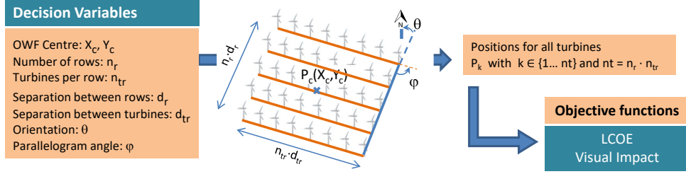
Figure 2: Parameters defining an individual. Eight parameters define the position for all of the OWF turbines. Once obtained the turbine positions, the objective functions can be evaluated.
