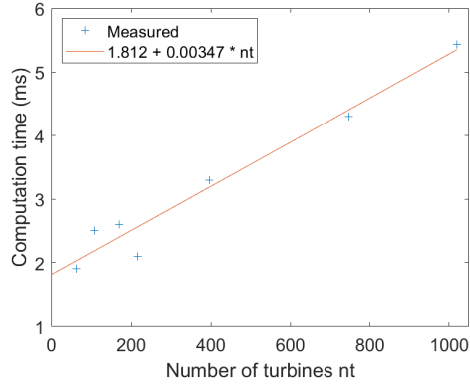
Figure 4: Time to compute the energy yield as a function of nt
