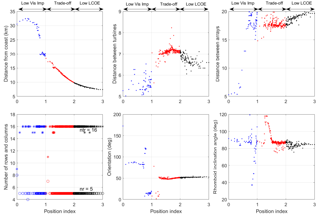
Figure 13: Distribution of parameters defining the individuals that compose the Pareto front. For each plot, the first third of points (in blue) corresponds to the quasi-horizontal curve with LOW VI; the second one (in red) is a transition zone; and the last third (in black) represents the solutions with low LCOE.
