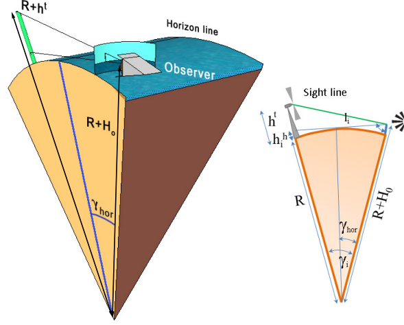
Figure 7: Representation of distances and angles between observer, horizon line and turbine
