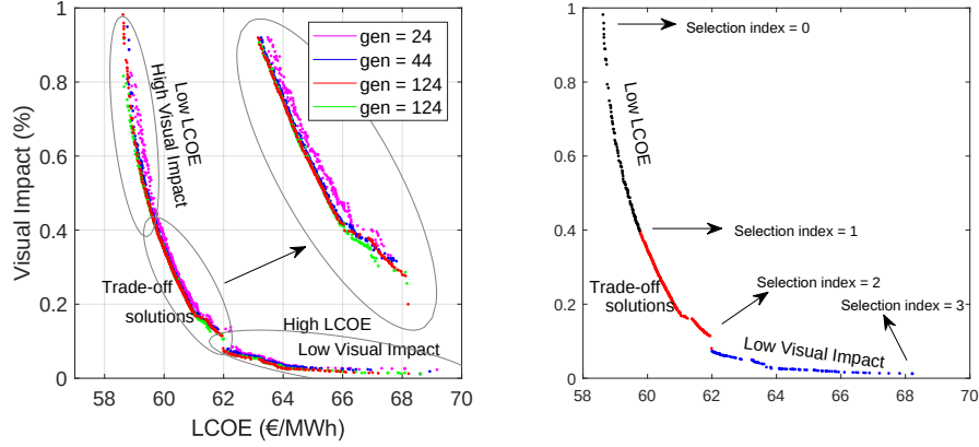
Figure 12: Evolution of the fronts using NSGA II technique and division into three zones (left-hand plot); final Pareto front using colours to visualize the three zones (right-hand plot).
