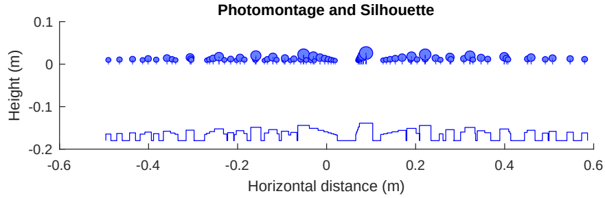
Figure 9: Representation of the turbines along the horizon line and merged occupation of the FoV. A distance to canvas equal to one has been used for the representation.
